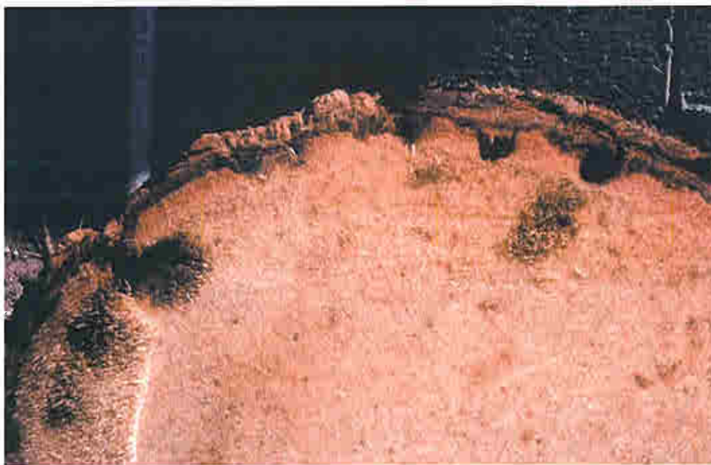
3. Section of the base of a stem of Phoenix canariensis infected with Fusarium oxysporum f.sp. canariensis .
